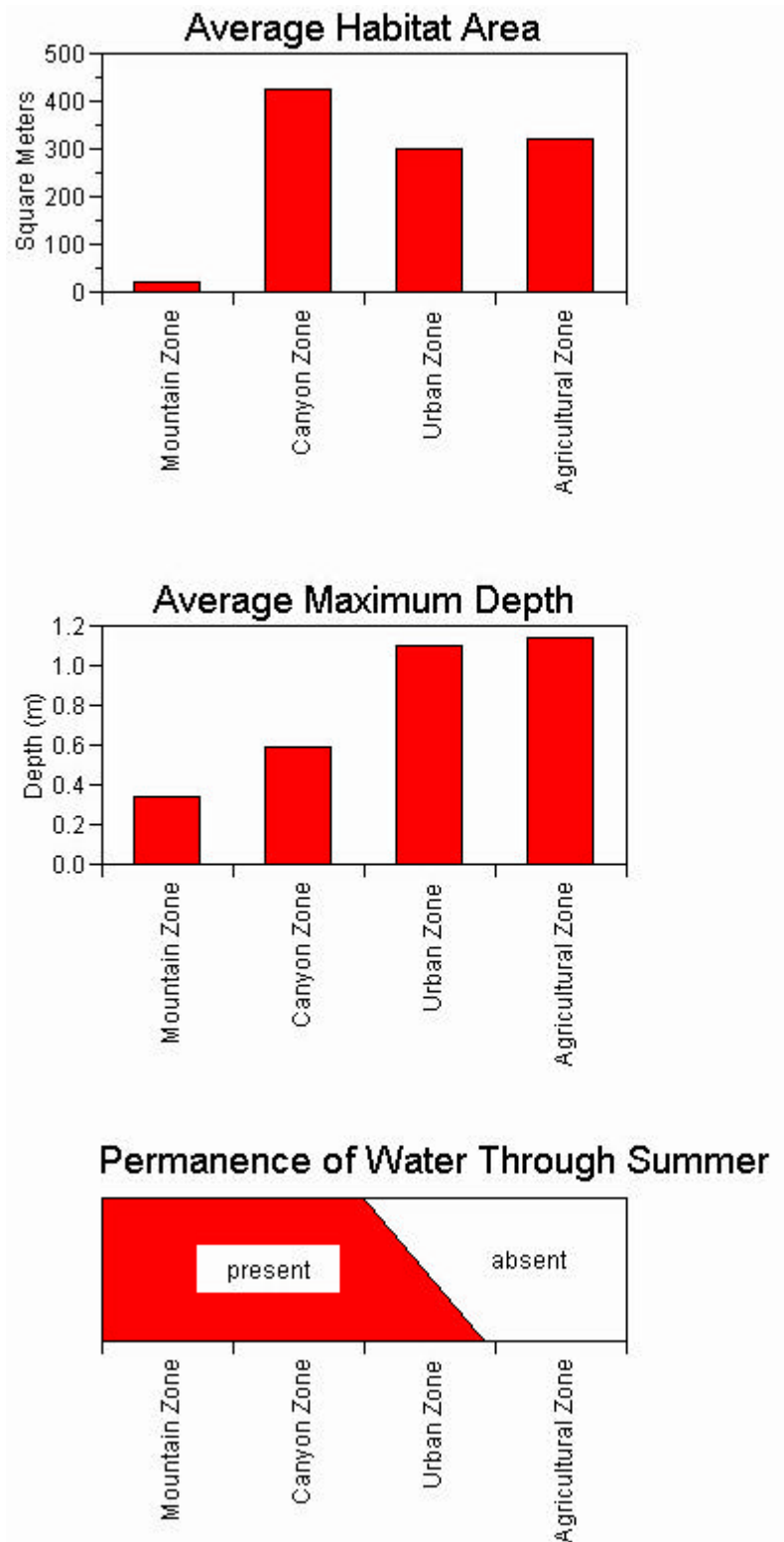
Figure 2.16. Selected habitat characteristics
