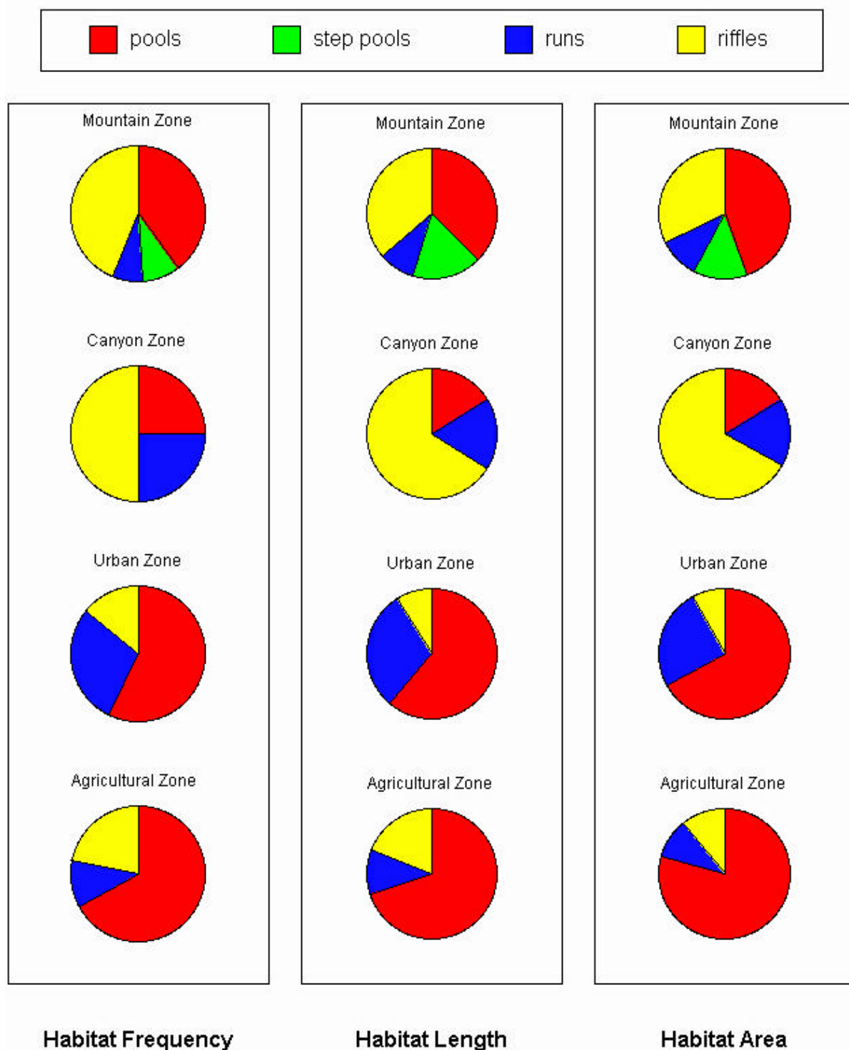
Figure 2.13. Distribution of fish habitat in Little Chico Creek
